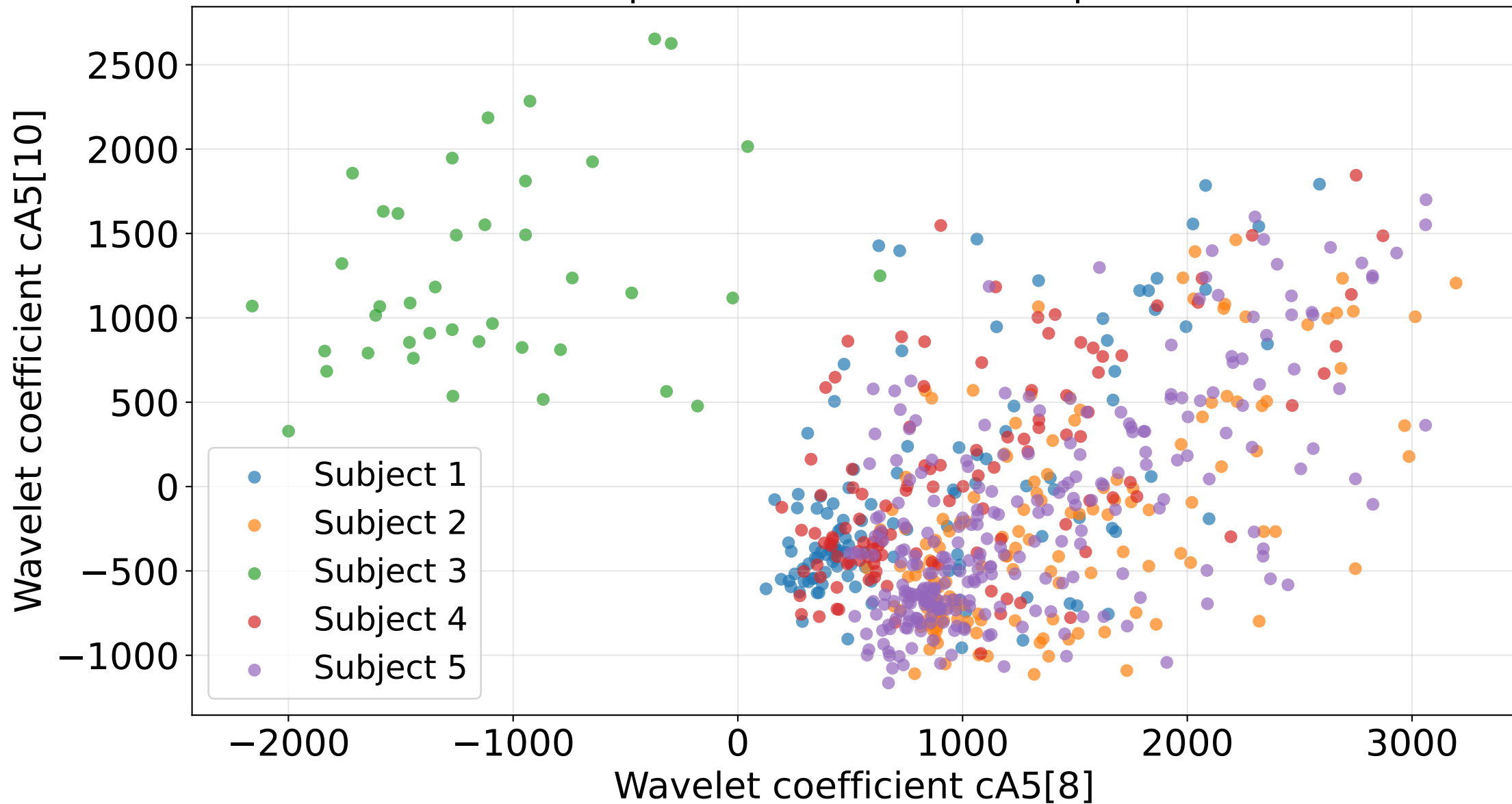
Ground-truth labels in the space of the two most important wavelet coefficients
